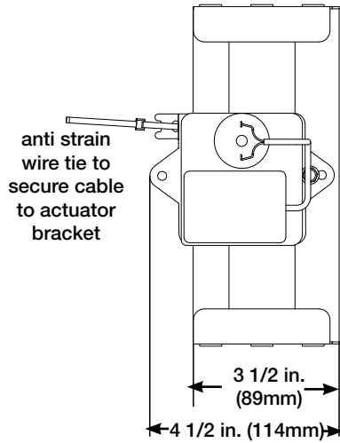
Side view Actuator field installed.
