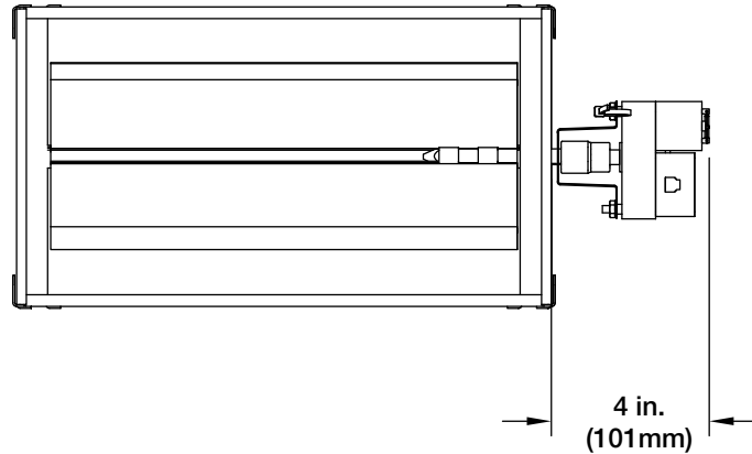
Front view Actuator field installed
