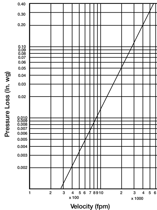
Pressure Drop 12 in. (305mm) dia. Damper
