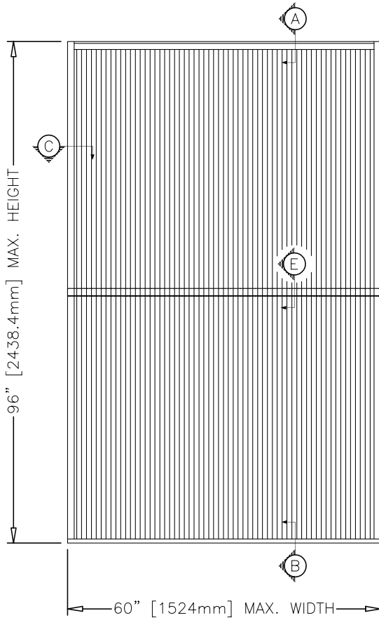
SINGLE SECTION W/ SUPPORT ANGLE
