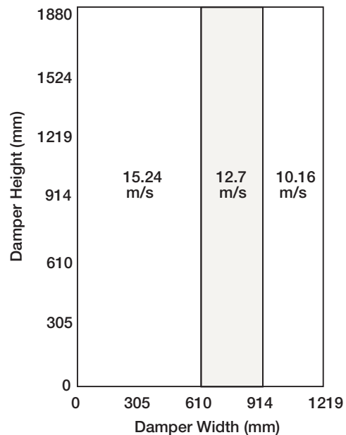
Velocity Limitations
