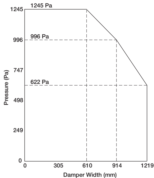
Pressure Limitations
