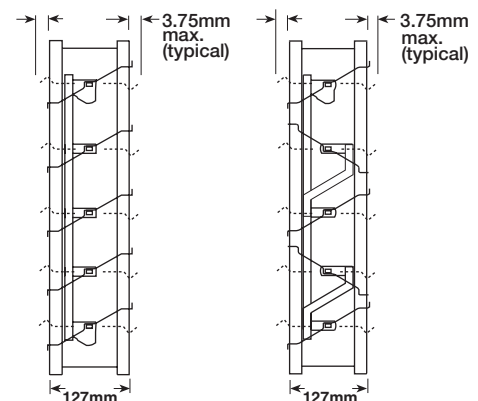
Parallel Blades
