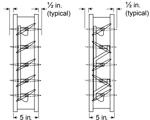
Parallel Blades
