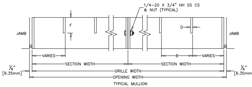
HORIZONTAL SECTION
