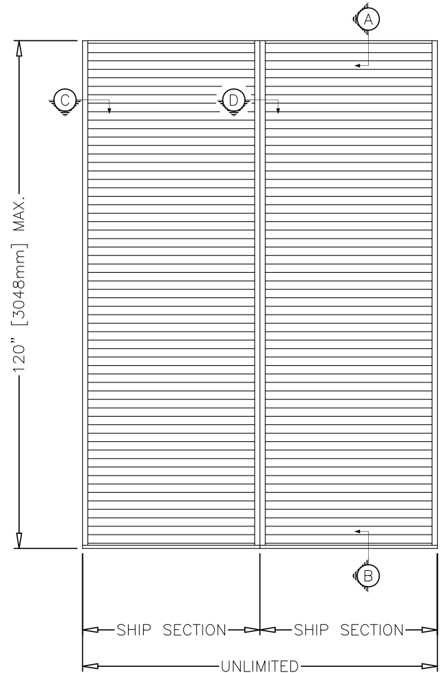
MULTIPLE SECTION W/ MULLION
