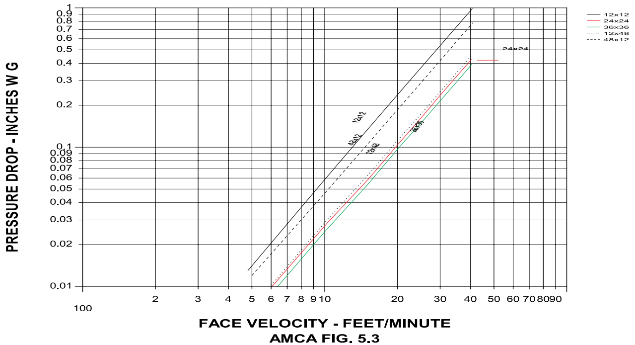
VELOCITY VS. PRESSURE DROP*
