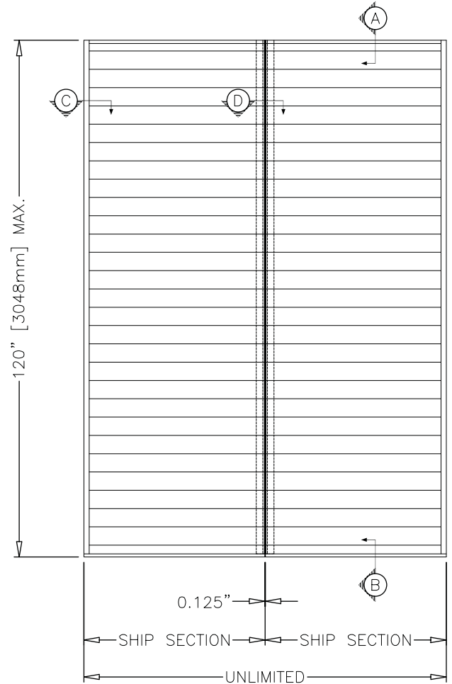
MULTIPLE SECTION W/ RECESSED MULLION
