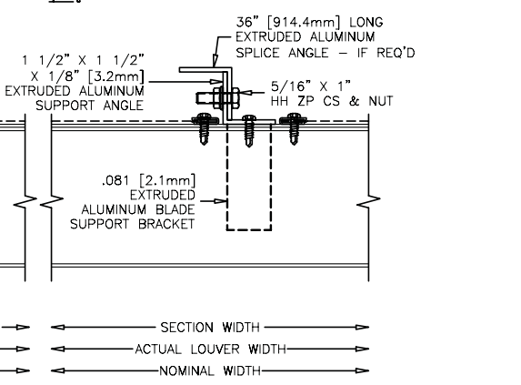
E SUPPORT DETAIL
