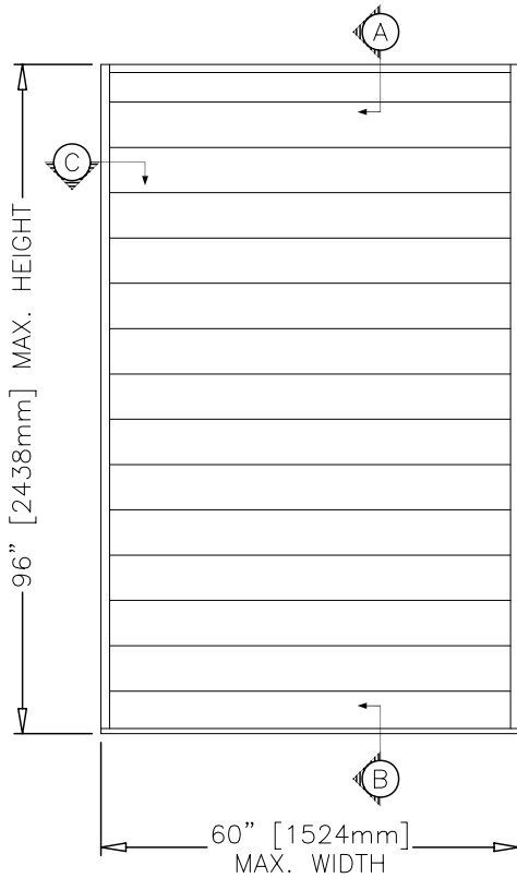
SINGLE SECTION
