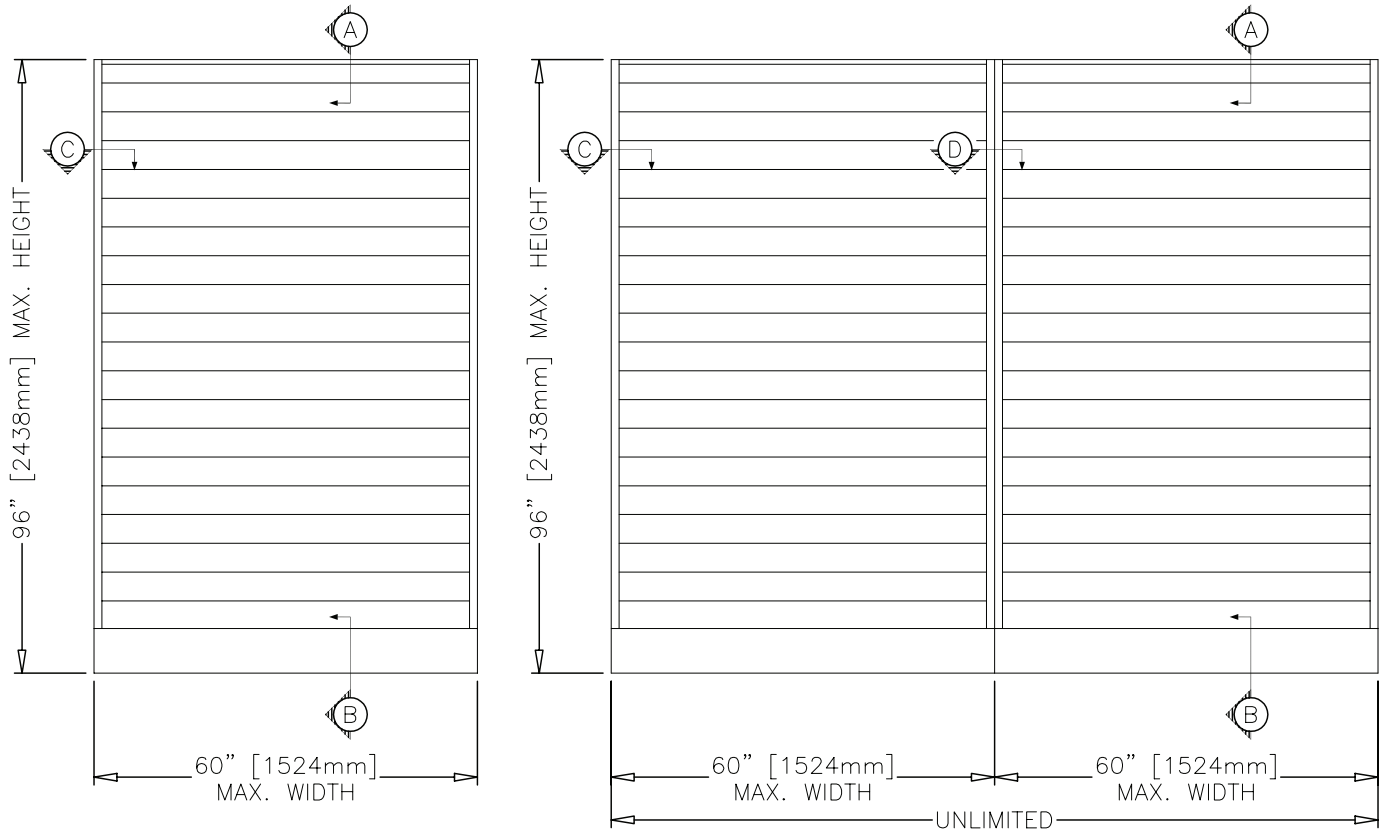
MULTIPLE SECTION W/ MULLION
