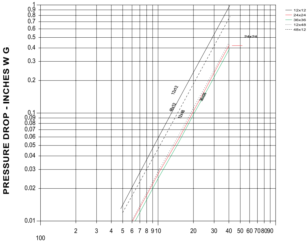
FACE VELOCITY - FEET/MINUTE AMCA FIG. 5.3
