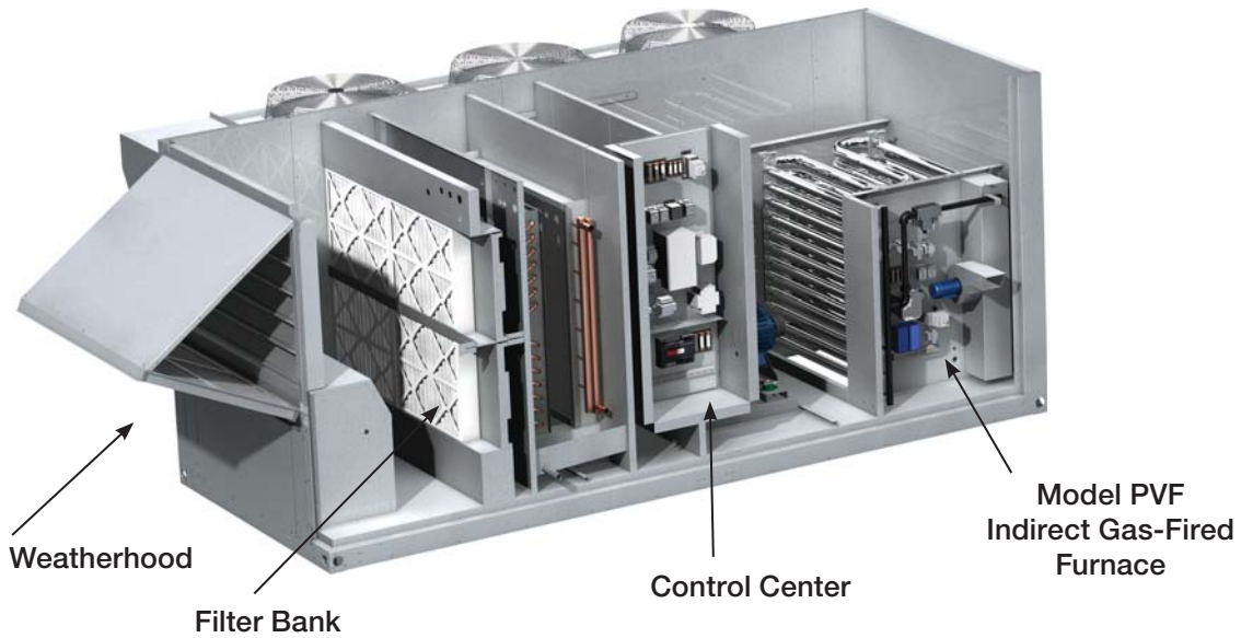
Model MPX - Open View
