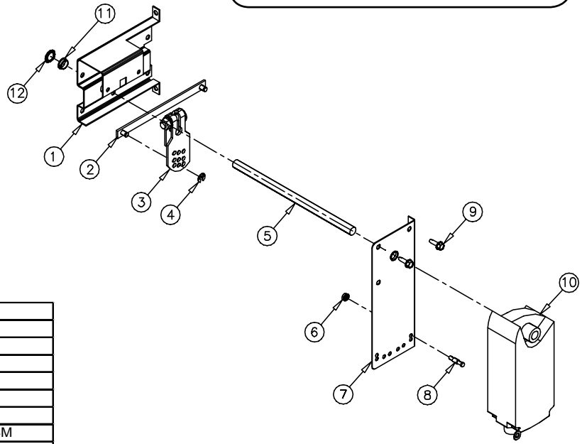
Figure 1: Siemens Series internal mount (exploded view).
