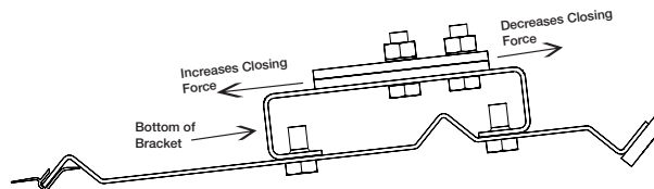
Figure 6: Counterweight adjustment in the full open position
