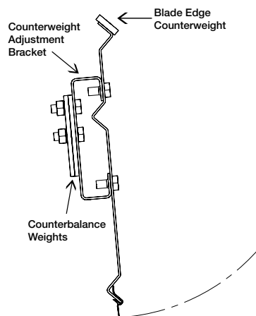
Figure 7 - Adjustable counterweight assembly detail
