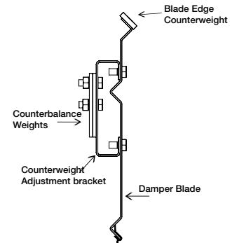
Figure 5 - Adjustable counterweight assembly detail
