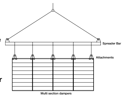
Figure 1- supports for lifting a multi-section damper
