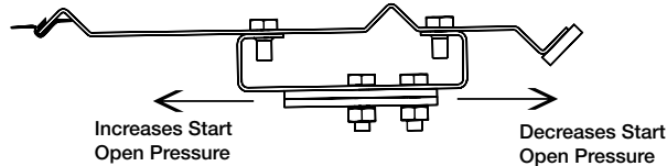
Figure 4: Counterweight adjustment for start open pressure. Blade is shown in full close position
