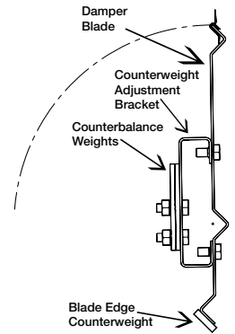
Figure 3 - Adjustable counterweight assembly detail
