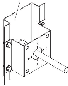
Orientation of Stand Off Bracket for a directly driven damper
