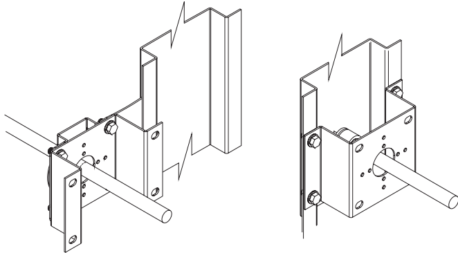
Orientation of Stand Off Bracket for a directly driven damper
