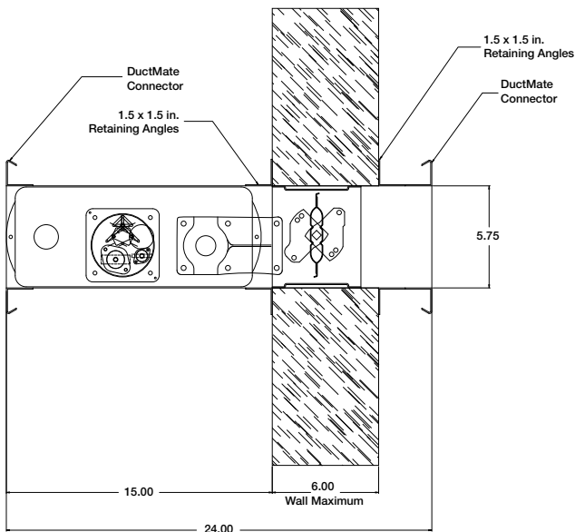
Figure 1: Smoke detector mounting orientation for dampers less than 25 inches (635mm) in height.
