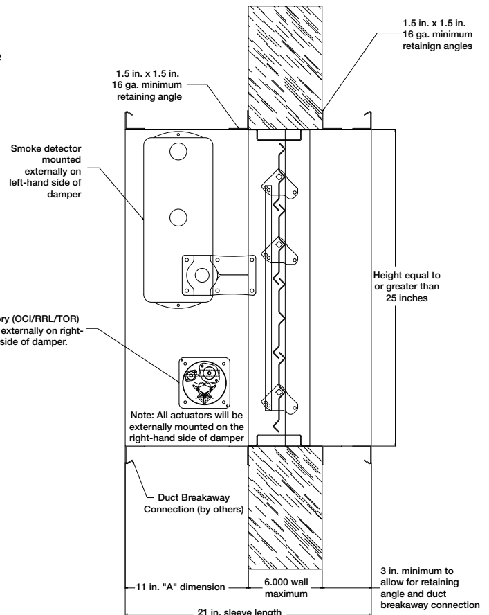
Figure 2: Smoke detector mounting orientation for dampers equal to or greater than 25 inches (635mm) in height.
