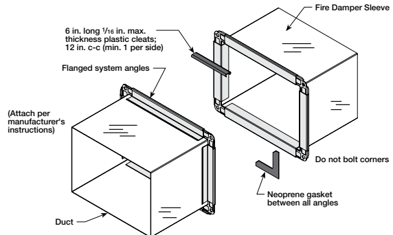
Figure 6: Detail of manufactured flanged system breakaway connections.
