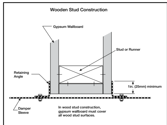
Figure 9: Detail of retaining angles and gypsum board application for metal and wooden stud construction.
