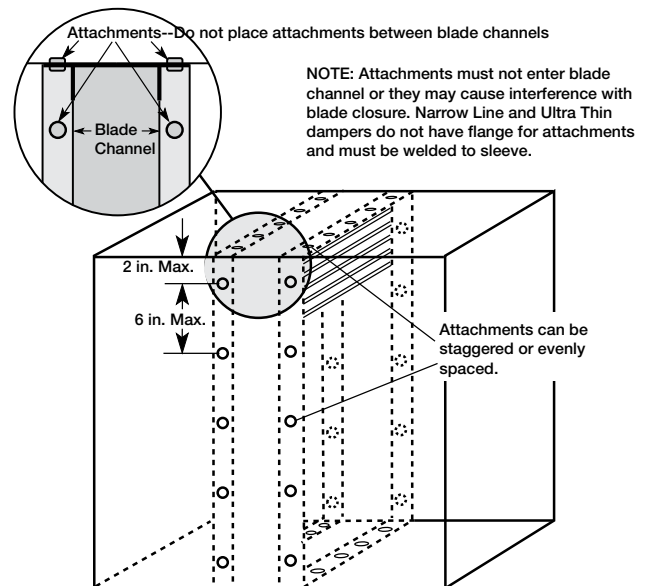
Figure 3: Field attachment of fire dampers to sleeves.
