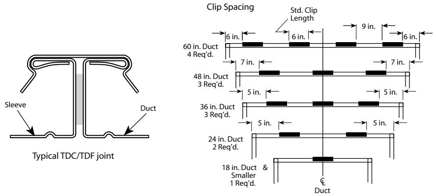
Figure 7: Detail of proprietary flanged system breakaway connections.
