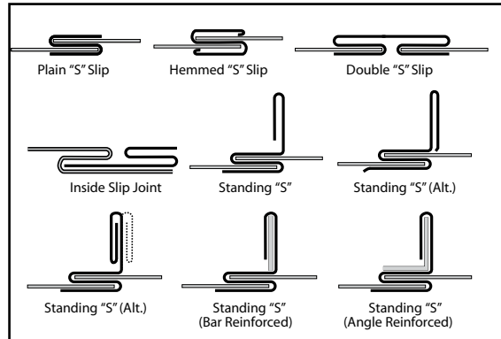
Figure 5: Traditional breakaway style transverse joints.
