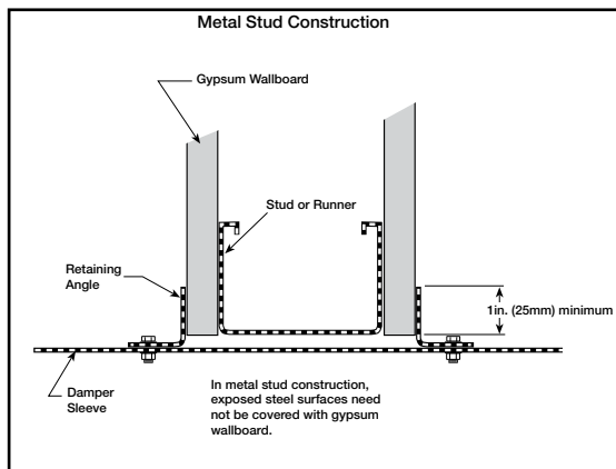
Figure 9: Detail of retaining angles and gypsum board application for metal and wooden stud construction.
