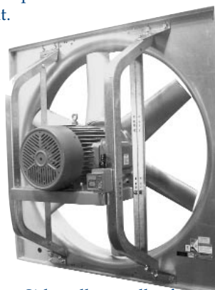
Sidewall propeller fans commonly use a dust-tight NEMA 4 disconnect.
