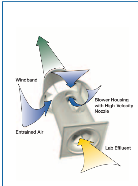
Figure 1: Induced flow inline mixed flow fan
